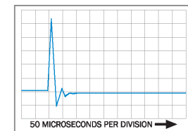
Impulse Response
