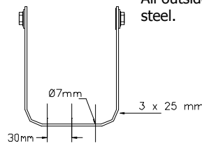
Optional Bracket Stainless steel
