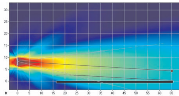
BeamWare display of an IC8R illustrating the reduced grating offered by ICONYX "A" series arrays with their improved algorithms and dual dome HF tweeters.
