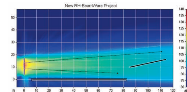
Beamware display of an Iconyx IC8A array's dual beam output..
